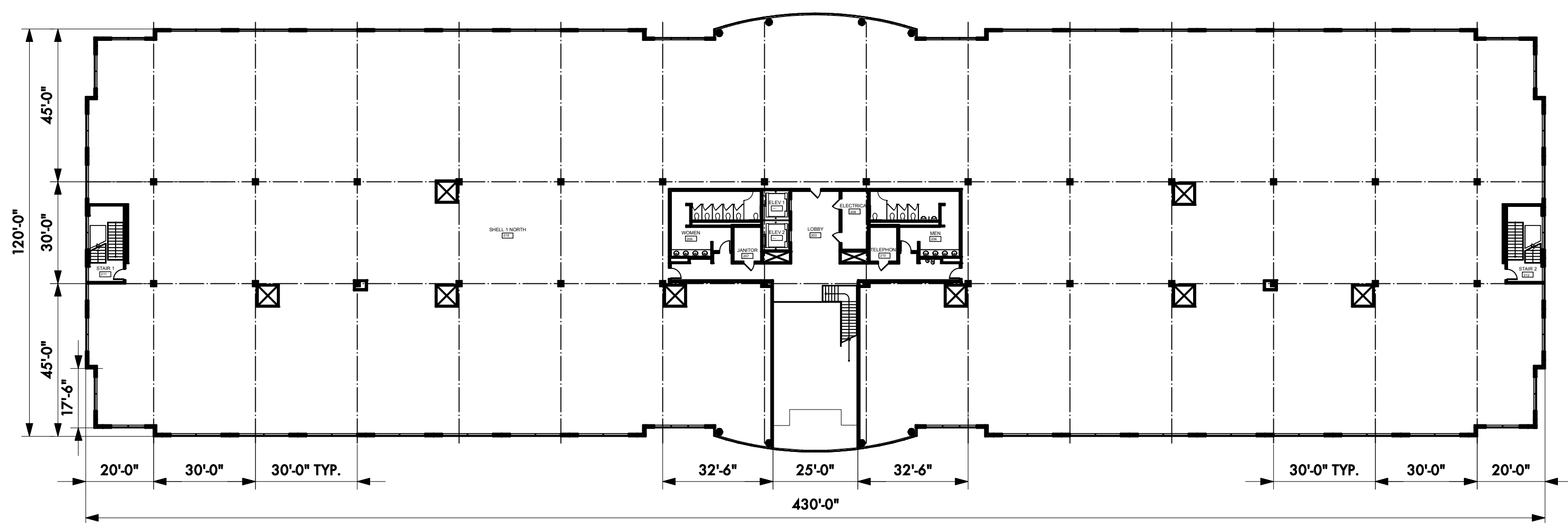
Second Floor 51,395 sf
