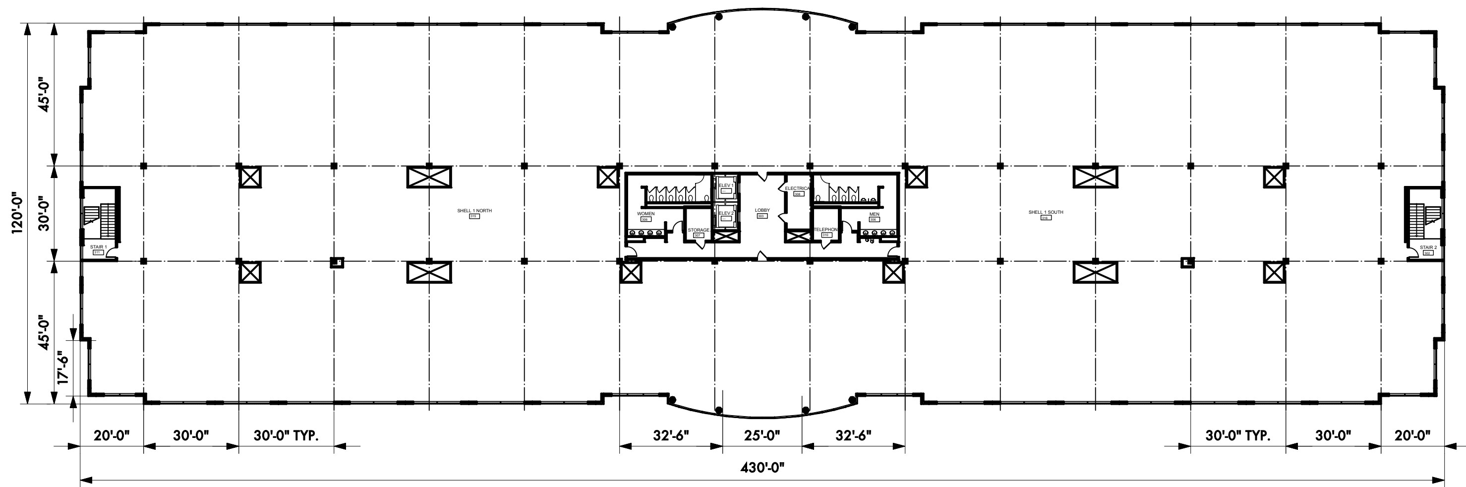
Third Floor 51,395 sf
