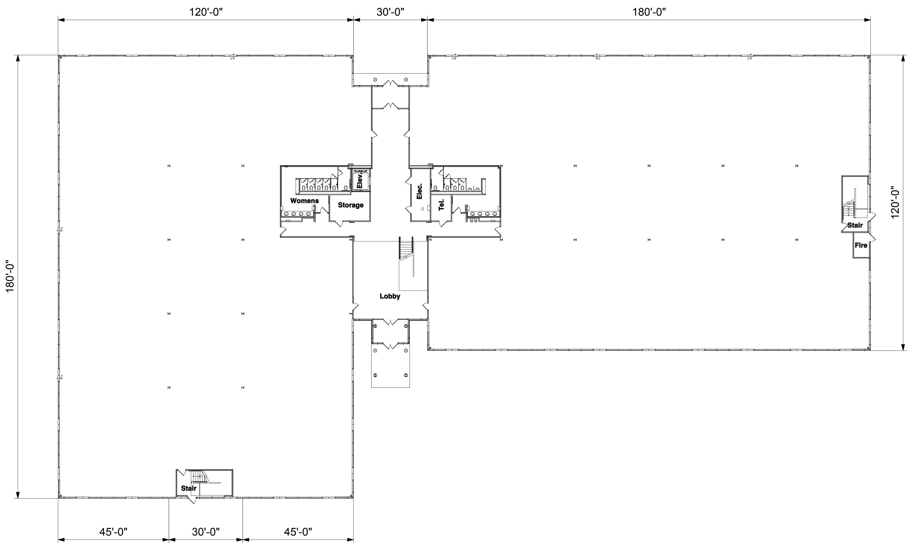
First Floor 46,200 gsf
